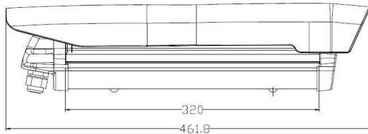
DIMENSION
